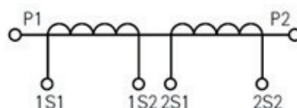
Double winding
